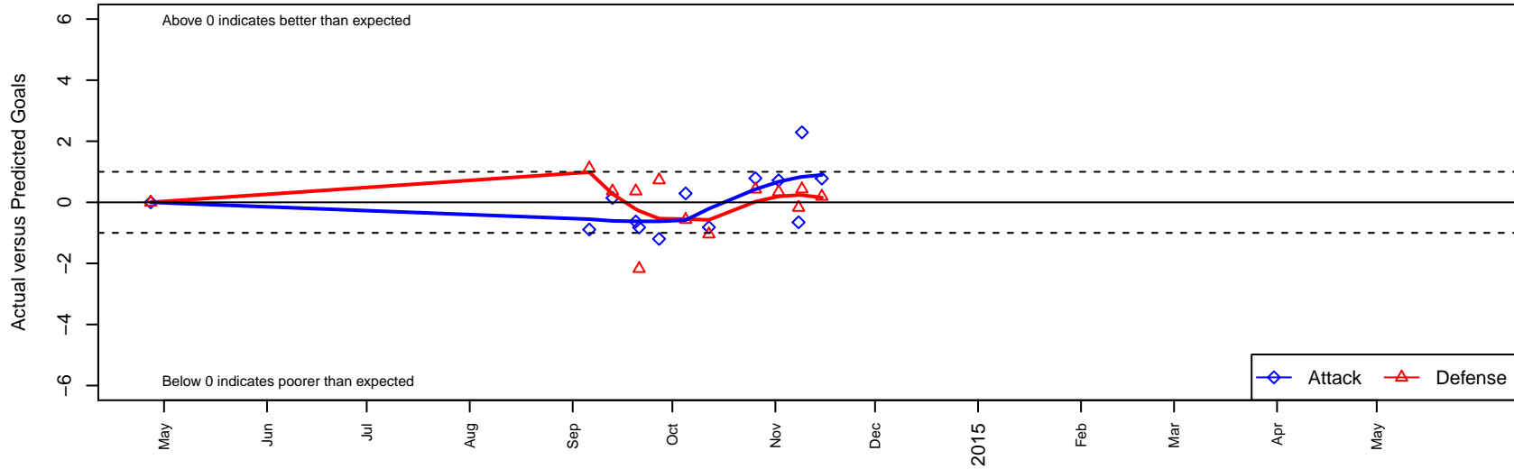
TVSA Hawks Academy B98 Dots are actual minus expected GF (blue circles) and GA (red triangles). Blue line is smoothed change in attack strength. Red is smoothed change in defense strength.
